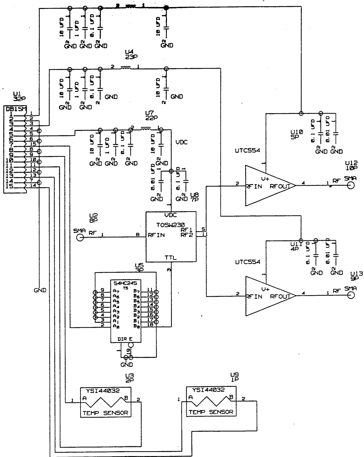
Figure 29 RF LNA Circuit Schematic
