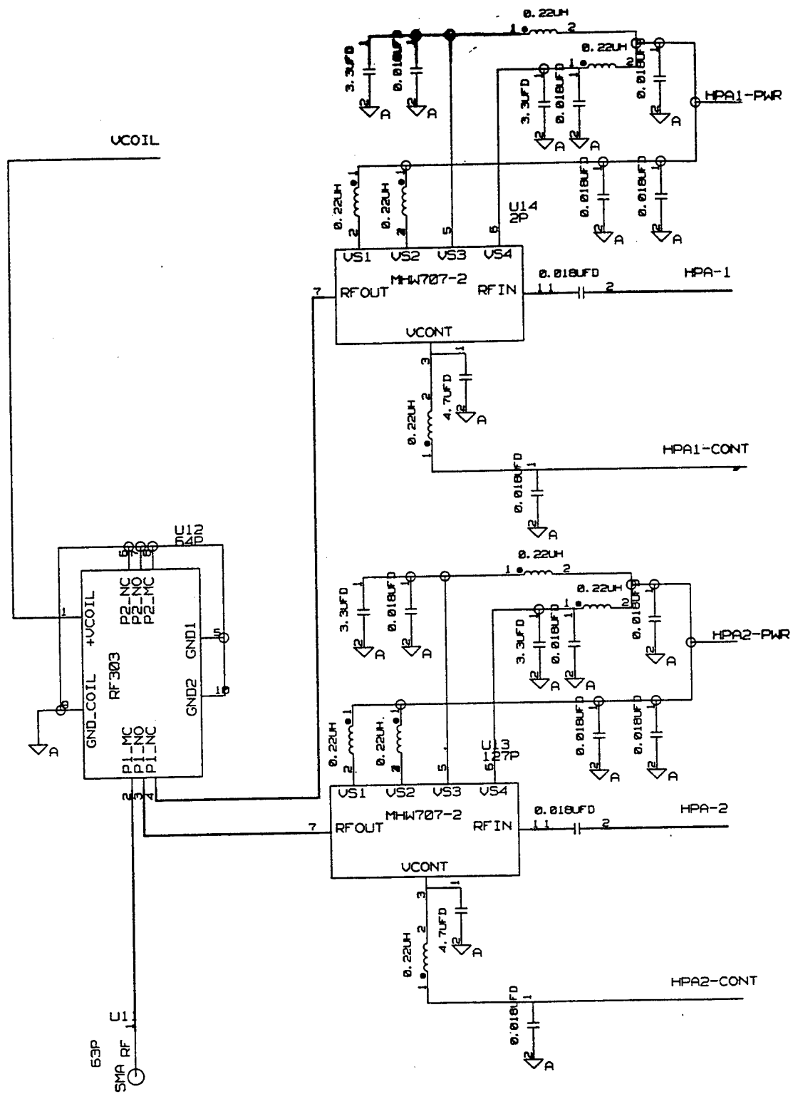
Figure 39 RF HPA Circuit Schematic- Output Section
